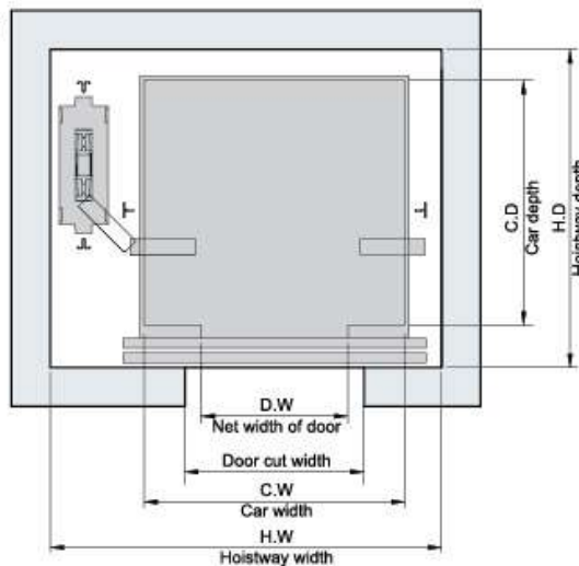
Hoistway plan
