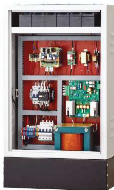
AUTOMATIC RESCUE DEVICE
