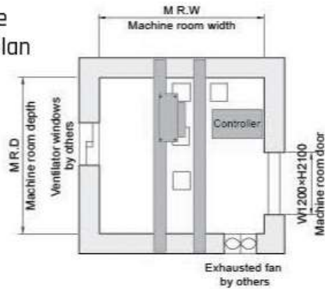
GRPS20 Small Machine room elevator specification
