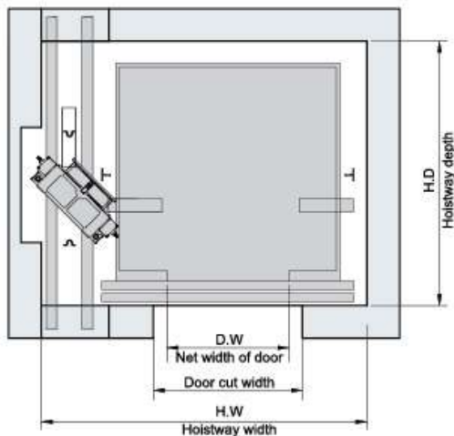
GRPN20 Machine roomless elevator specification
